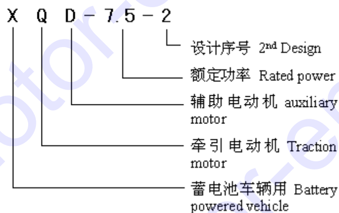
DC auxiliary motor
