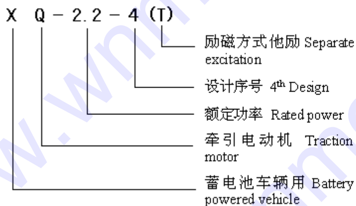
DC traction motor
