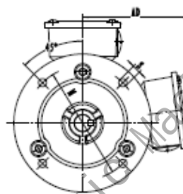
H63-200mm
